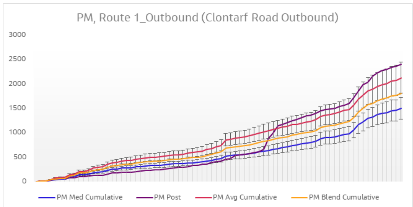
Diagram 6.23 Journey Time Validation Plot - Route 1 Outbound PM
