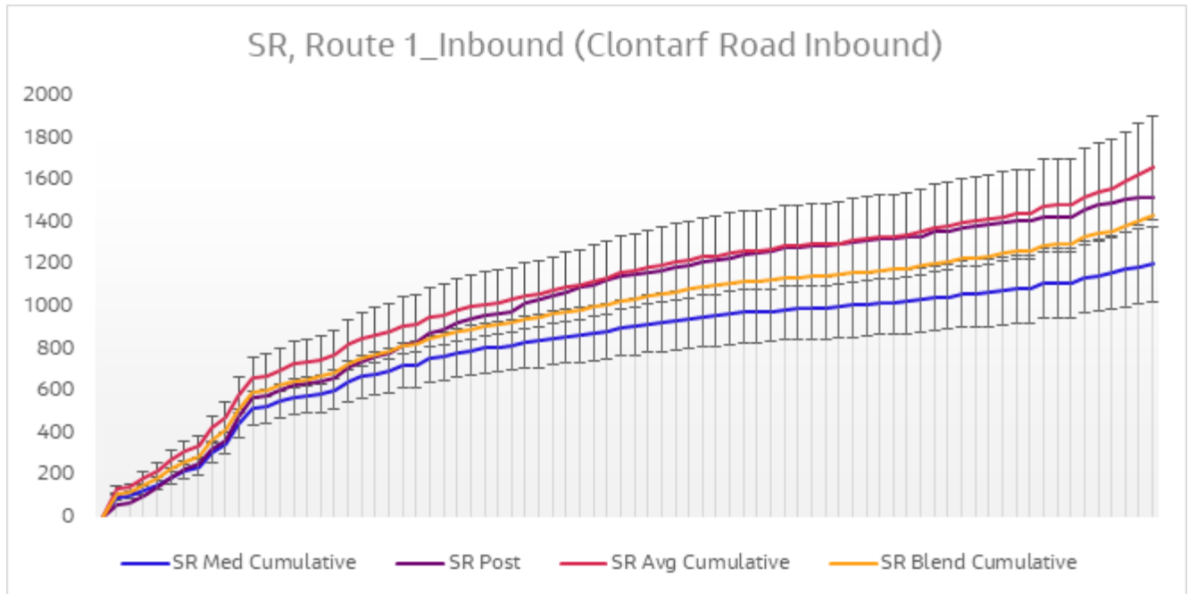
Diagram 6.18 Journey Time Validation Plot - Route 1 Inbound SR
