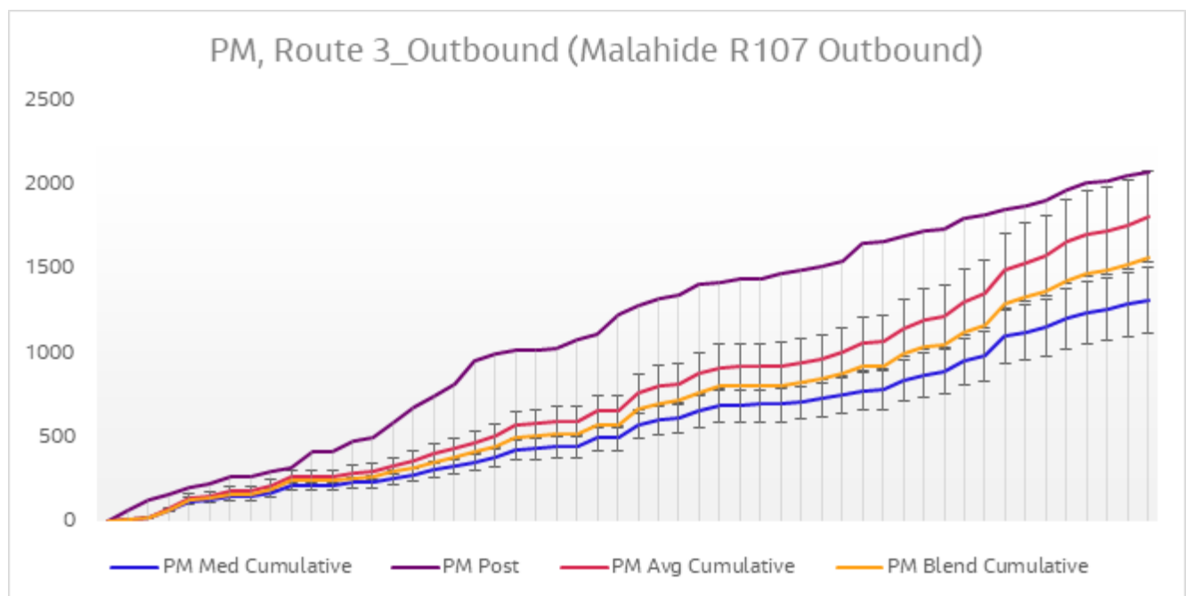
Diagram 6.25 Journey Time Validation Plot - Route 3 Outbound PM
