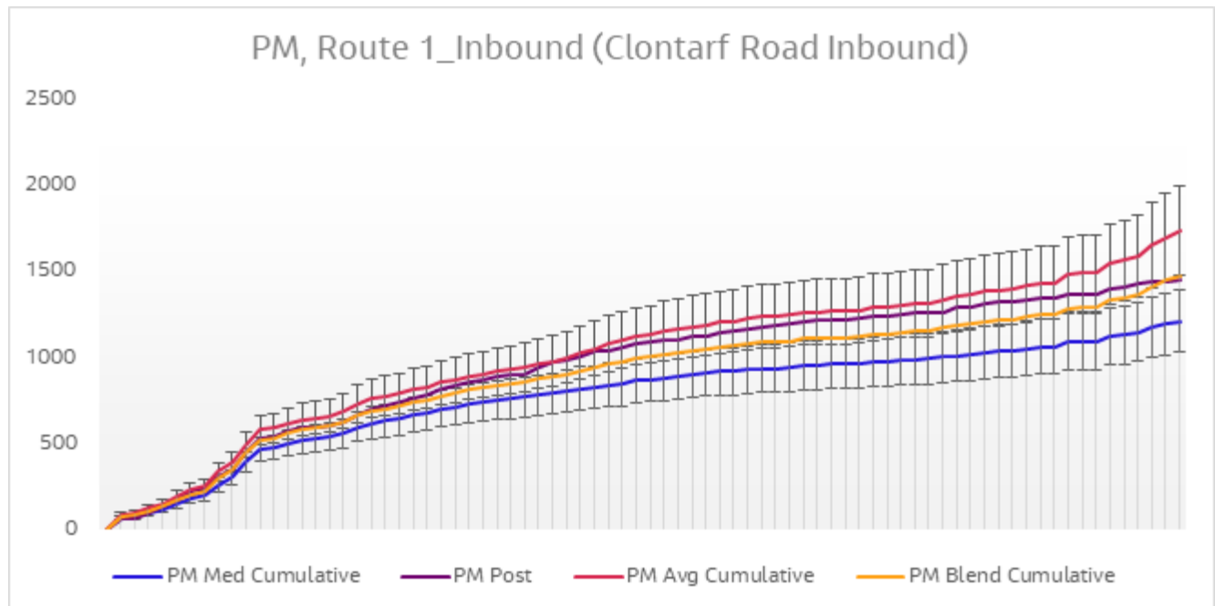
Diagram 6.22 Journey Time Validation Plot - Route 1 Inbound PM
