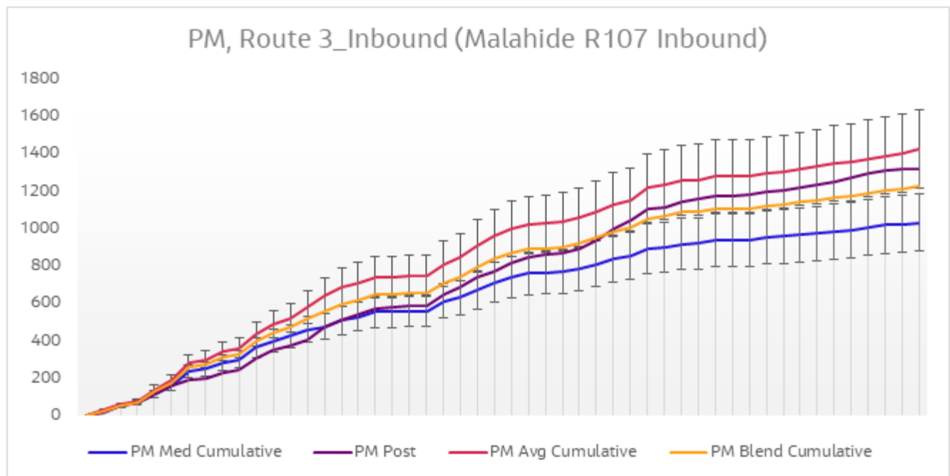
Diagram 6.24 Journey Time Validation Plot - Route 3 Inbound PM
