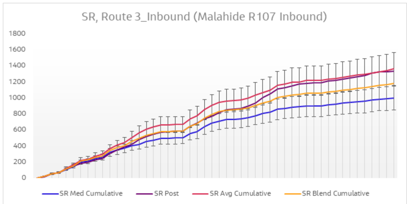
Diagram 6.20 Journey Time Validation Plot - Route 3 Inbound SR
